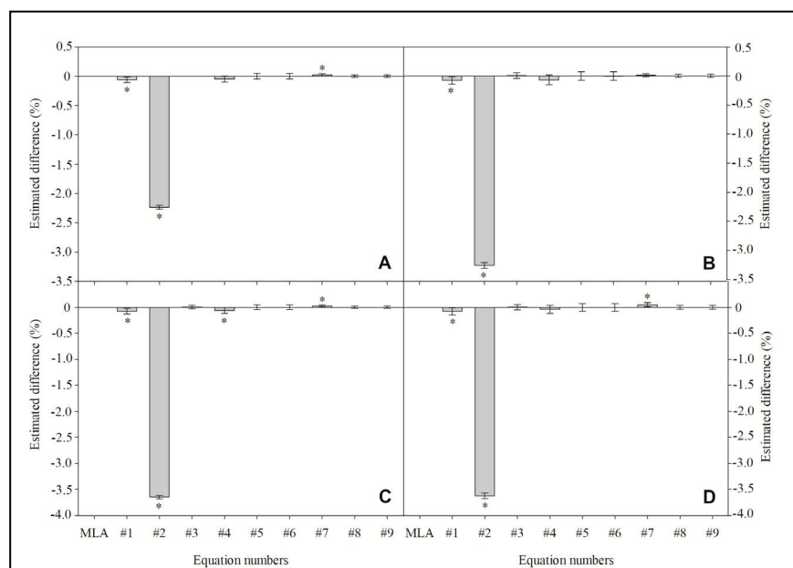
Figure 1. Deviation of the estimated area from the observed leaf area (LAo) for individual leaves. Leaf areas for the genotype 4 (A), 16 (B), 18 (C), and Morita II (D) of Stevia rebaudiana were estimated using several models in which \beta_0 and \beta_1 are coefficients. Vertical bars denote means and spreads denote 99% confidence intervals of the difference (distribution of t-test). For details of the equations and its equation number, see Table 2. The asterisks (*) denotes biased equations. Cordoba, University of Cordoba, 2020.
