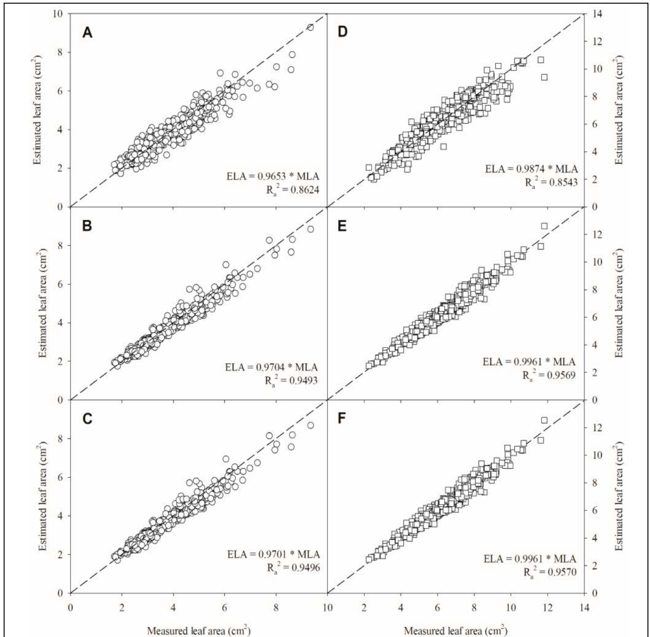
Figure 3. The relationship between estimated and measured area for the Stevia rebaudiana leaves. Leaf area was estimated in accord of equations #3 (A, D), #8 (B, E), and #9 (C, F) for genotype 4 (A-C), and genotype 16 (D-F) (for more details of these equations, see Table 2). Dotted line represents the 1:1 relationship. n = 500. Cordoba, University of Cordoba, 2020.
