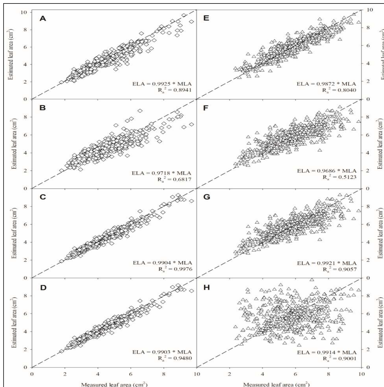
Figure 4. The relationship between estimated and measured area for the Stevia rebaudiana leaves. Leaf area was estimated in accord of equations #3 (A, E), #6 (B, F), #8 (C, G), and #9 (D, H) for genotype 18 (A-D), and Morita II (E-H) (for more details of these equations, see Table 2). Dotted line represents the 1:1 relationship. n = 500 . Cordoba, University of Cordoba, 2020.
