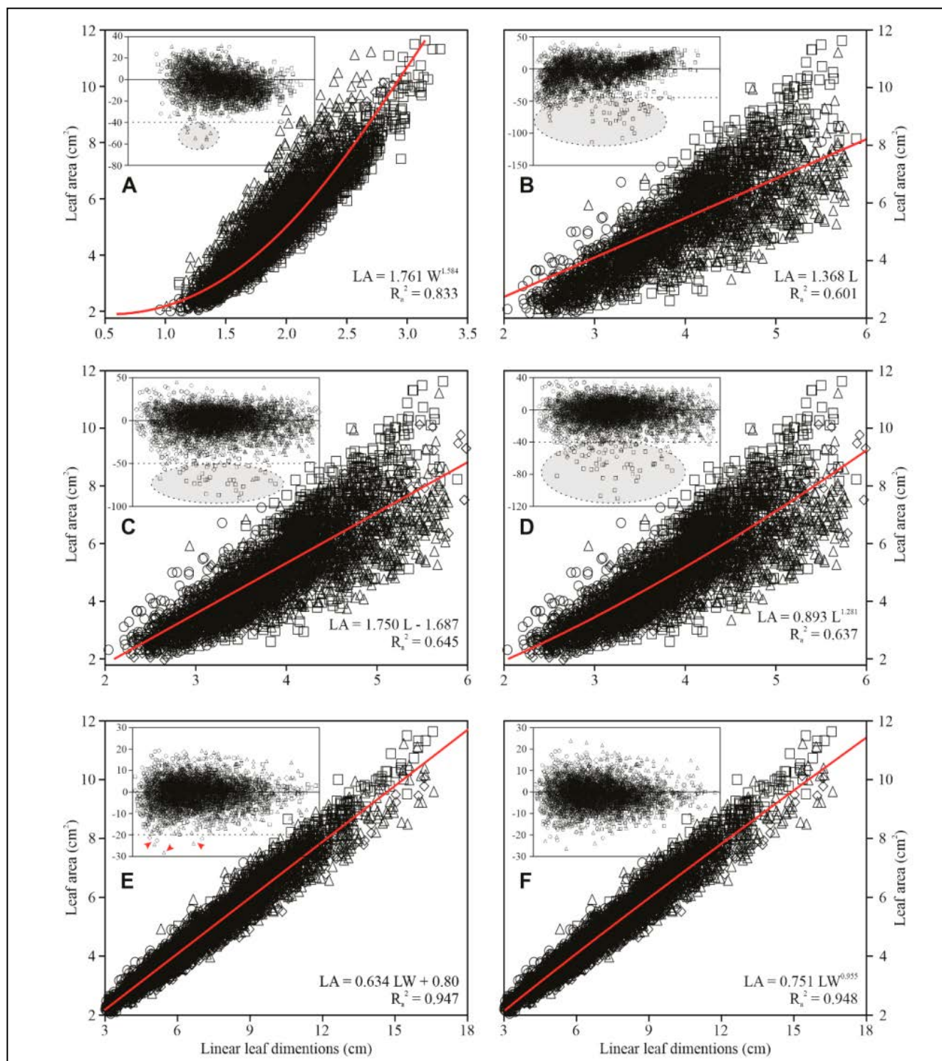
Figure 2. Regression curves for leaf area and linear leaf dimensions: width (A; equation #3), length (B-D; equation #4, #5, and #6), and product of leaf width and leaf length (E-F; equations #8, and #9) for Stevia rebaudiana leaves: Genotypes 4 (circles), 16 (squares), 18 (diamond), and Morita II (triangle), using linear (B, C, and E) and power (A, D, and F) models. The dispersion pattern of residuals for the respective models is shown in the insets. The shaded area denotes the region of highly biased data in the equations causing an overestimation of Stevia rebaudiana leaves, while data pointed with arrows denote a slight overestimation of Stevia rebaudiana leaves. All graphs were generated with 1,000 independent leaves of each Stevia rebaudiana genotypes. Cordoba, University of Cordoba, 2020.
